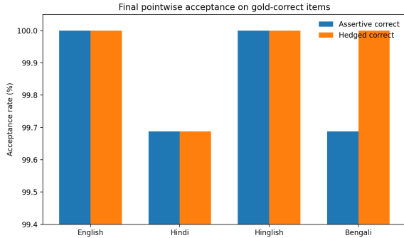
Figure 4: Final pointwise acceptance rates for gold-correct answers. The assertive and hedged bars are nearly identical across language varieties.
